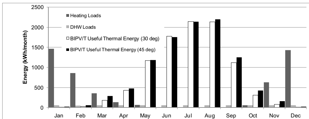
Figure 7: Comparison of thermal loads and BIPV/T useful energy output
