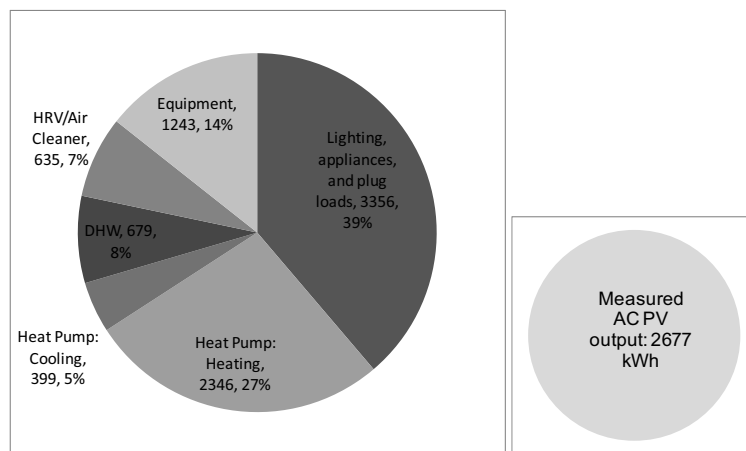
Figure 5: a) projected annual electricity loads by use. b) measured PV electricity generation. Areas are proportional to energy values, which are all in kWh.
