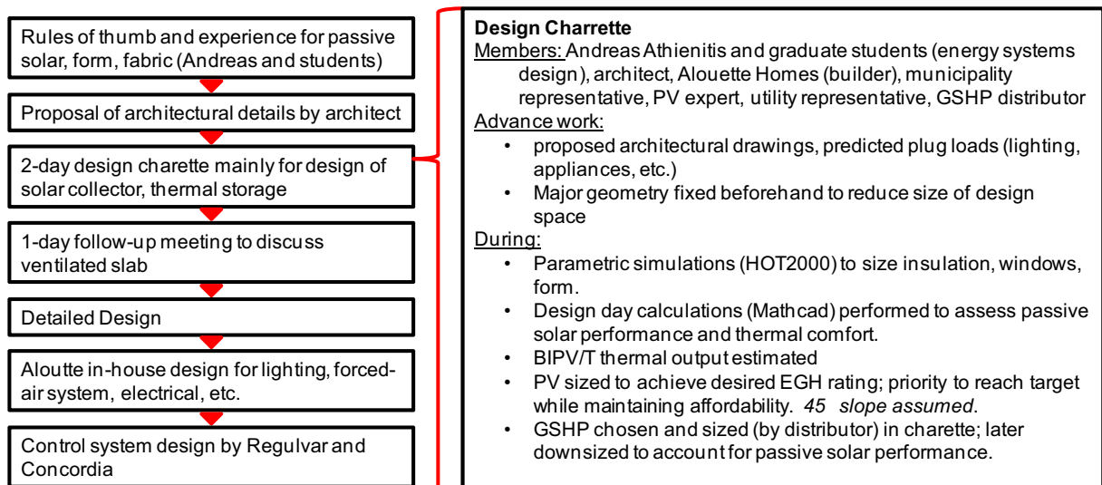
Figure 2: Design process outline
