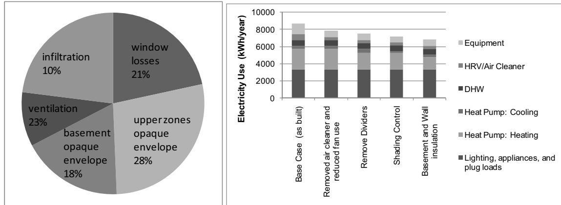
Figure 6: a) distribution of total heat loss during the heating season; b) electricity use for successive upgrades
