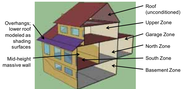
Figure 3: a) Select model inputs; b) section view of thermal model with zoning scheme.
