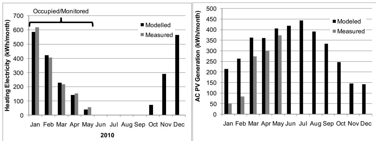
Figure 4: Comparison between the model and measured performance for: a) heating energy consumption and b) PV electricity generation
