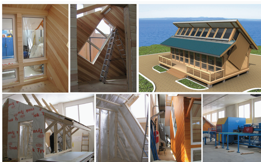
Fig.5. “EcoModule Solar-5M” under construction in “Technopark” FENTU.
