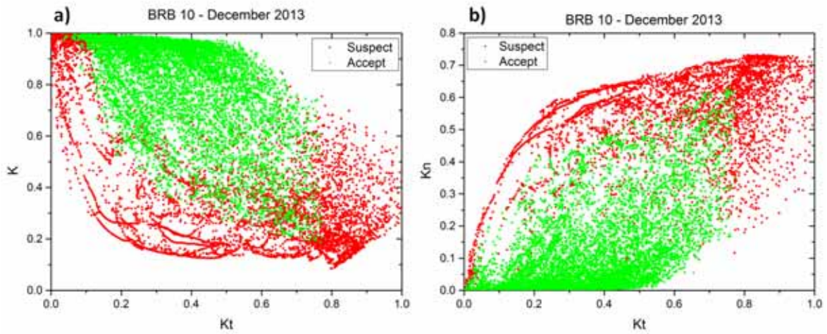
Fig. 6: Preliminary results provided by QC algorithm performed for data files acquired at Brasília (10) to a) K vs. K_t and b) K_n vs. K_t .
