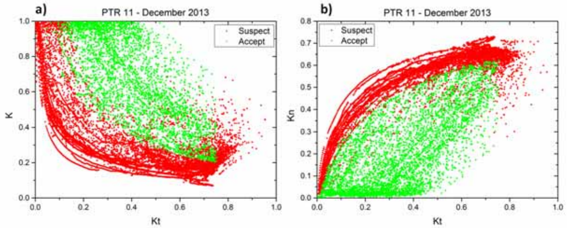
Fig. 5: Preliminary results provided by QC algorithm performed for data files acquired at Petrolina (11) to a) K vs. K_t and b) K_n vs. K_t .
