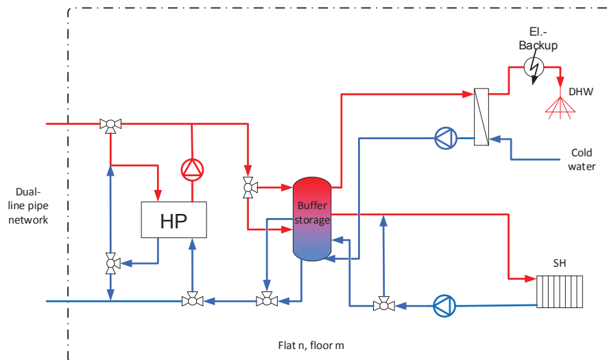
Fig. 5: Dual-line pipe network with decentralized heat pumps in each individual flat
