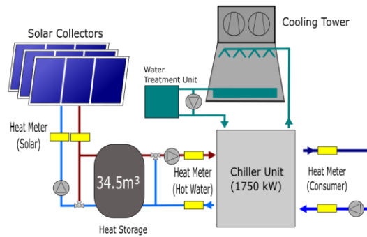
Fig. 3: Simplified hydraulic schema of DMHS.
