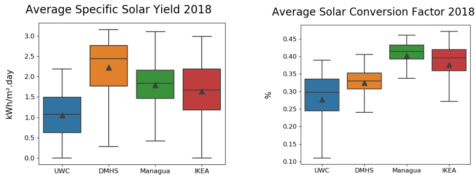
Fig. 13: Average specific solar yield (left) and average solar conversion factor (right) of each solar system in 2018. Median are displayed by a solid black line, quartiles are marked by colored boxes and the range of the measured data is displayed by the black whiskers. Averages are marked by black solid triangles.
