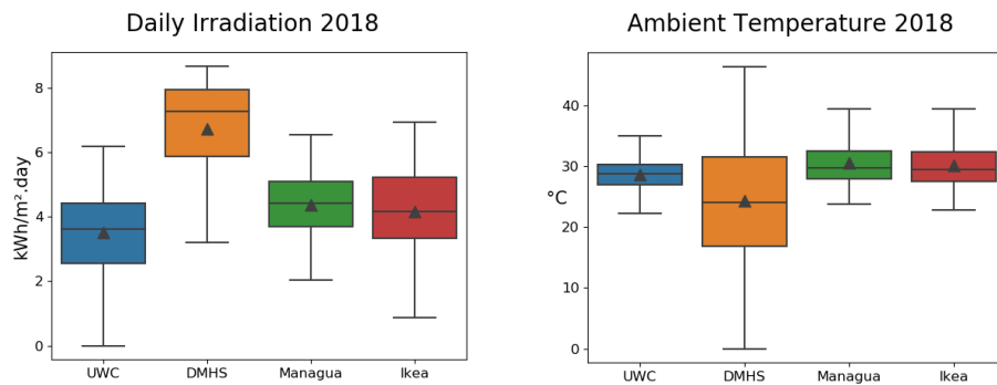
Fig. 11: Average daily radiation per day (left) and average ambient temperature (right) for each system in 2018. Black lines mark the median, the border of the colored boxes mark the quartile and the whiskers mark the range of the measured data. Average values are displayed by black triangles.
