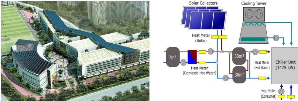
Fig. 1: Design view of the UWC campus with collector arrays in blue (left) and simplified hydraulic schema of UWC (right).
