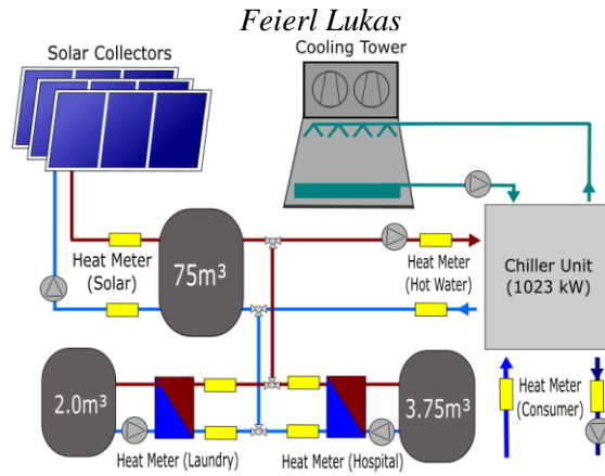
Fig. 5: Simplified hydraulic schema of MANAGUA.
