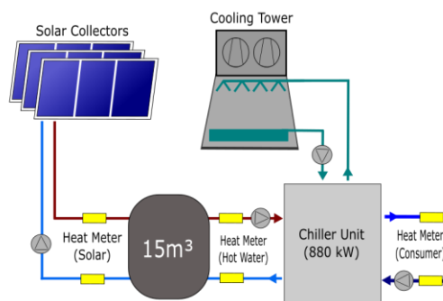
Fig. 7: Simplified hydraulic schema of IKEA.
