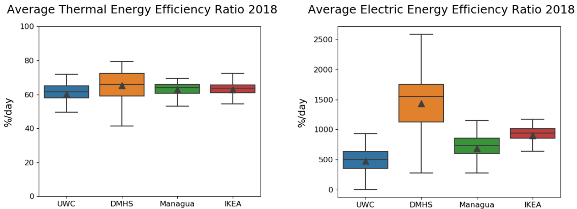
Fig. 14: Thermal (left) and Electrical Energy Efficiency Ratio (right) of each plant in 2018. Average values are displayed by black triangles, the median is displayed as horizontal line, the quartiles are marked by the colored boxes and the range of the calculated data is marked by the black whiskers.
