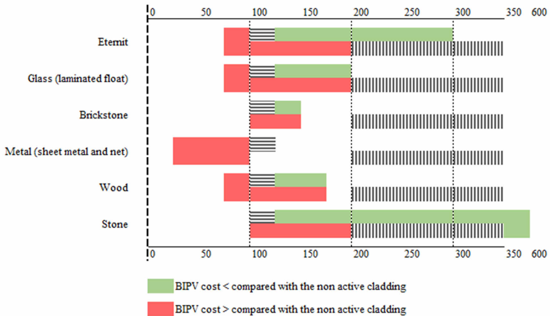
Fig. 11: Extra-cost BIPV compared with the material (CHF/m 2 )
