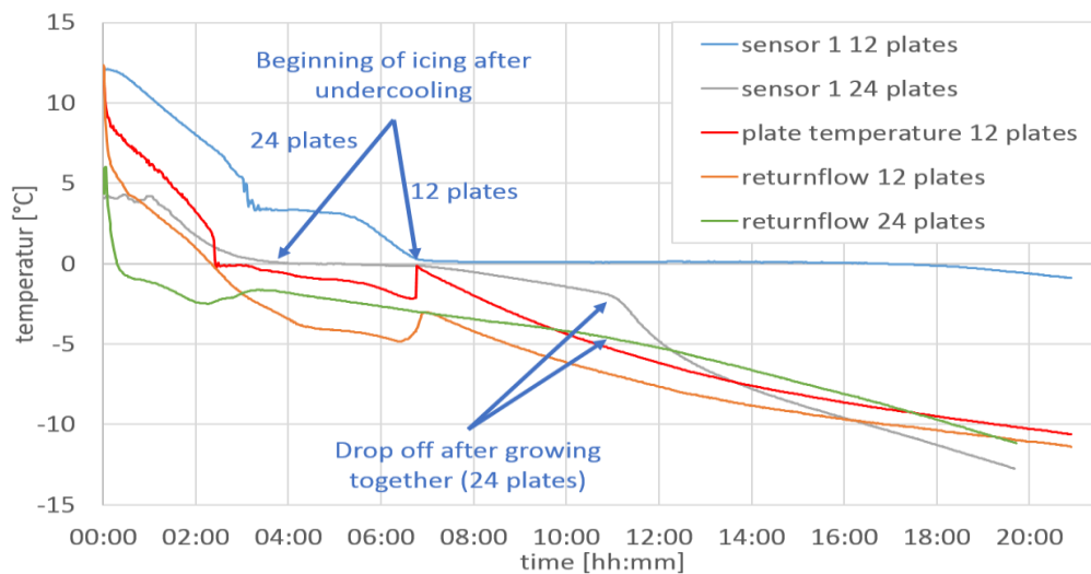
Fig. 12: Difference of the return flow temperatures of the primary circuit of the heat pump with 12 (yellow) and 24 (green) heat exchanger and of the temperatures between the plates (blue and grey)
