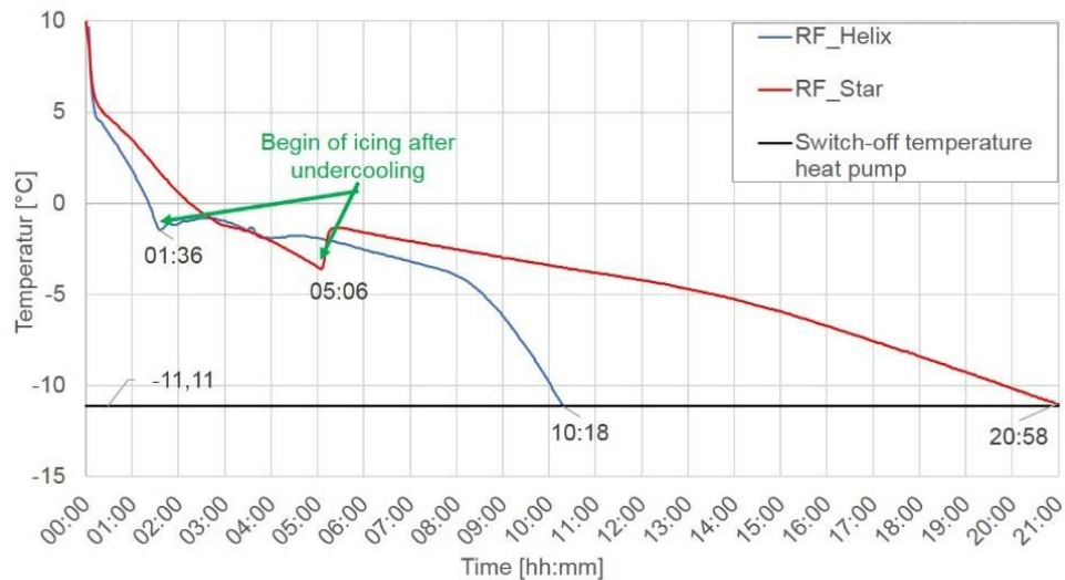
Fig. 9: Difference of the return flow temperatures of the primary circuit of the heat pump with helix (blue) and star-shaped (red) heat exchanger with 24 plates
