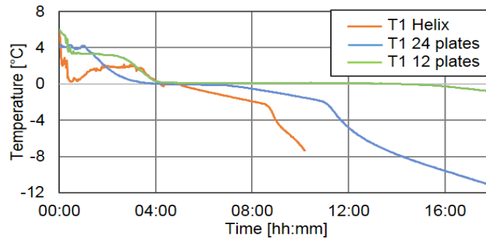
Fig. 11: Difference of the temperature profile of temperature sensor 1 with helical heat exchanger (orange), 24 plates (blue) and 12 plates (green) heat exchanger during the icing process
