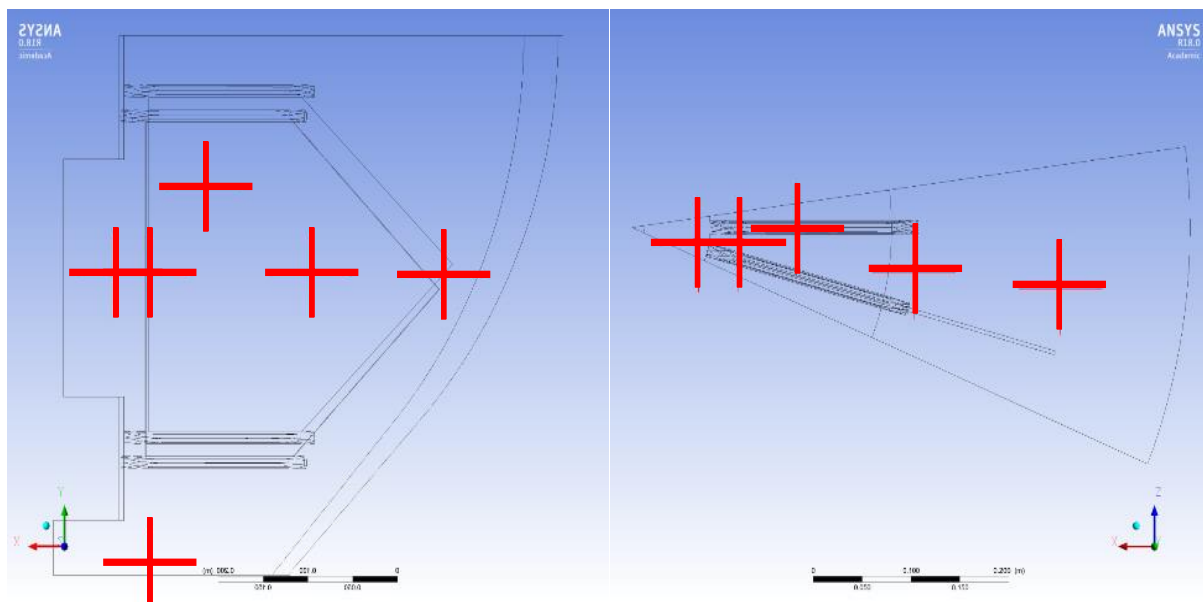
Fig. 4: Arrangement of the temperature sensors in the simulated part with two heat exchanger plates
