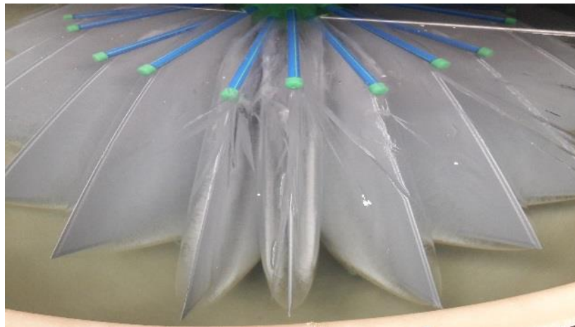
Fig. 8: Ice built-up after one icing cycle of the heat pump at the star shaped heat exchanger with 24 plates
