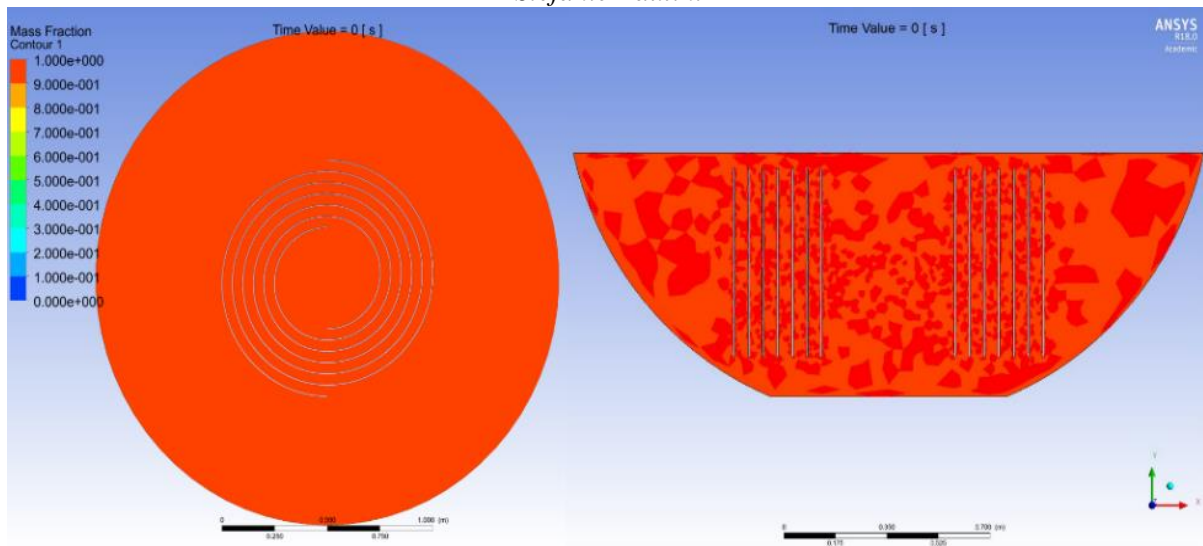
Fig. 3: Horizontal (left) and vertical (right) cut through the helix heat exchanger
