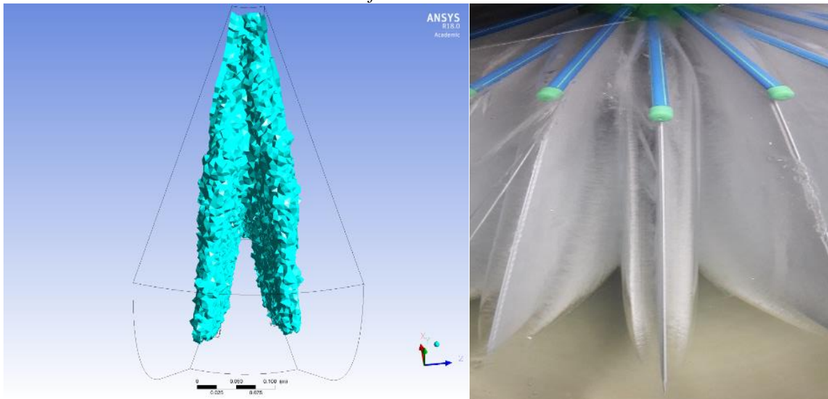
Fig. 13: Ice built-up in the simulation (left) and icing experiment (right) for the star-shaped heat exchanger with 24 plates
