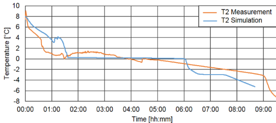
Fig. 5: Temperature profile of the model experiment (orange) and the simulation (blue) during the icing process
