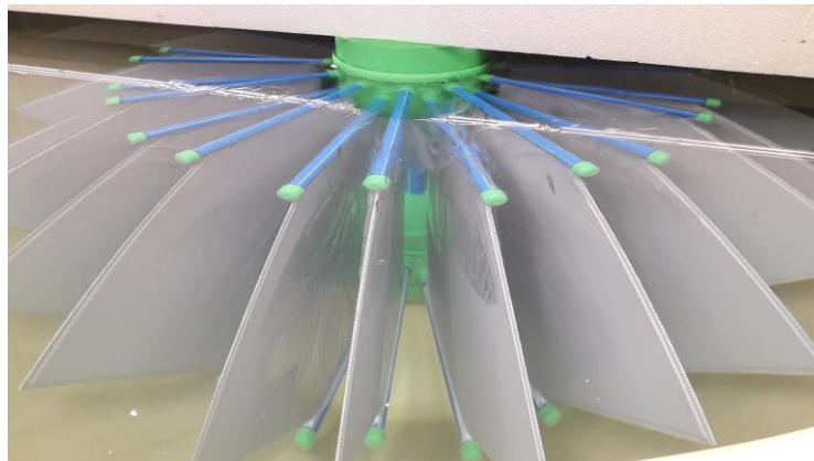
Fig. 6: Beginning of freezing at the star-shaped heat exchanger with 24 plates
