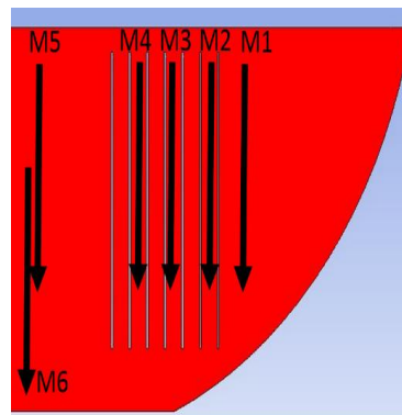
Fig. 2: Horizontal cut through the helix heat exchanger with points of temperature measurement
