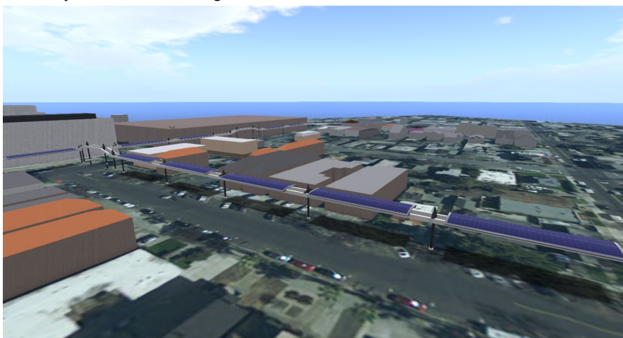
(Fig. 4) The Superway model in Encitra
