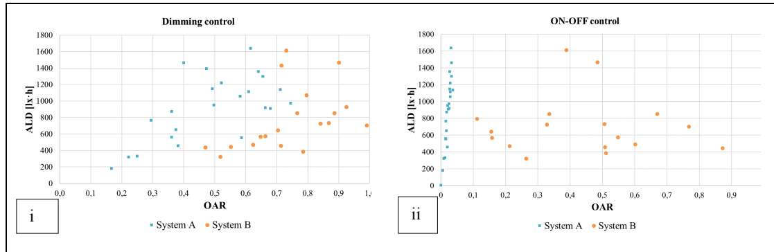
Fig. 6: Relationship between A.L.D and OAR indices calculated in dimming and ON/OFF control for the two systems.
