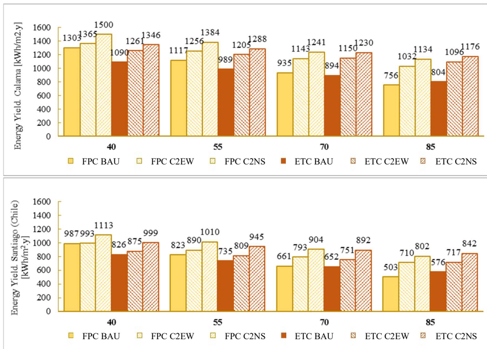
Fig. 7a: Energy yields [kWh/m 2 .y] by aperture area for different solar thermal BAU and ULISSES technologies and return temperatures for Calama (Chile) and Santiago (Chile).
