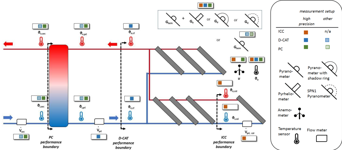
Fig. 8: System layout, sensor locations and performance boundaries
