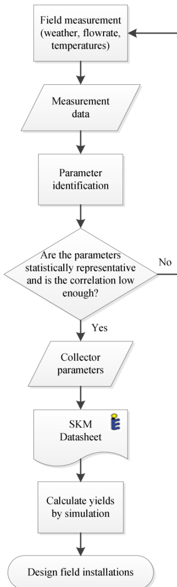
Fig. 1: Process diagram of a field certification measurement
