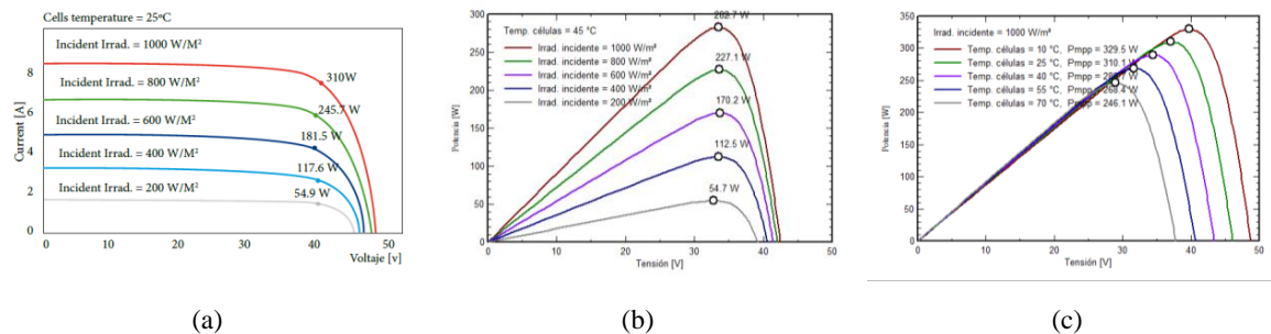
Figure 4. Curves for the characterization of the photovoltaic modules. (a) Performace curves by manufacturer (module Exiom Solution Poly 310 Wp 72 cells). (b) Influence of variations of the irradiance on the P-V curve (according PVsyst) (c) Influence of variations of the temperature, for a stable solar irradiance, on the P-V curve (according PVsyst).
