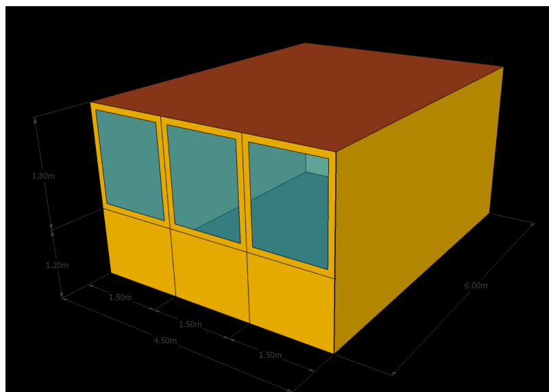
Fig. 1: View of the reference office zone.
