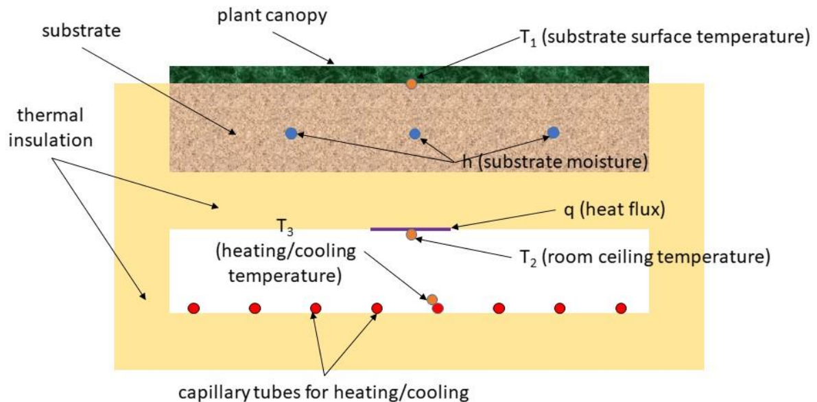
Fig. 4: Cross-sectional drawing of the measurement setup for the various roof structures and position of the individual sensors for temperature T , substrate moisture h , and heat flow q .
