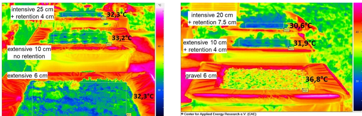
Fig. 10: Thermographic images of the six roof structures shortly after installation. Although the thermographic images were taken at a very shallow angle, reflections should have almost no influence on the results since the emissivity of all relevant surfaces (substrate, gravel, and leaves) typically are in the range of 90 % to 95 %.
