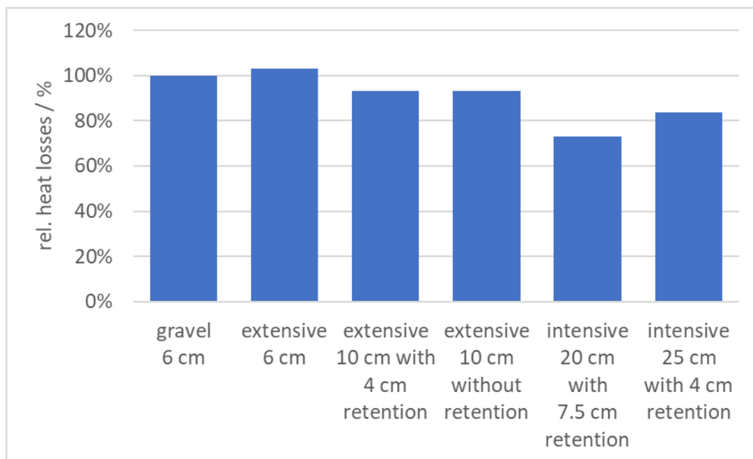
Figure 11: Measured relative heat losses of the green roof systems related to the heat input of the reference roof (set to 100 %) for the measurement period from October 15, 2023 to April 04, 2024.
