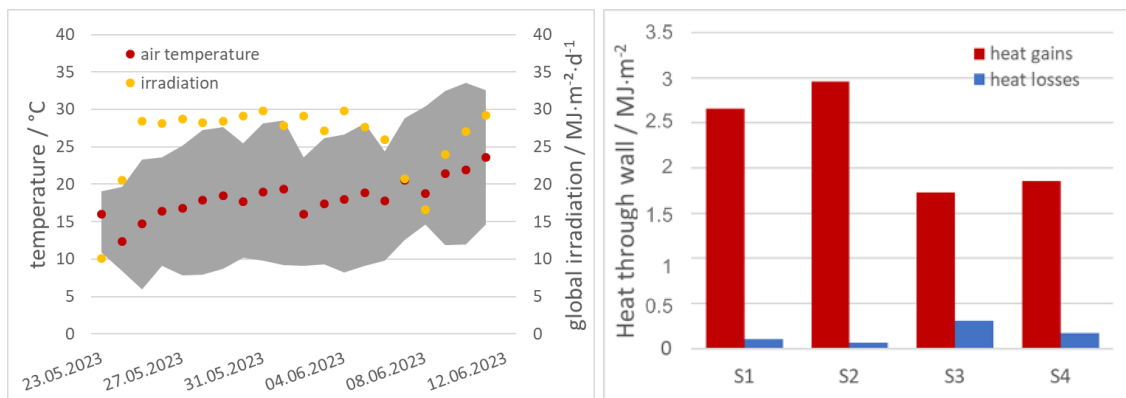
Fig. 5: Measured daily mean air temperature (red dots), minimum and maximum daily air temperature (grey area), and horizontal solar global irradiation (left); summarized heat gains and losses from May 23, 2023 to June 11, 2023 through the wall sections without LWS (right).
