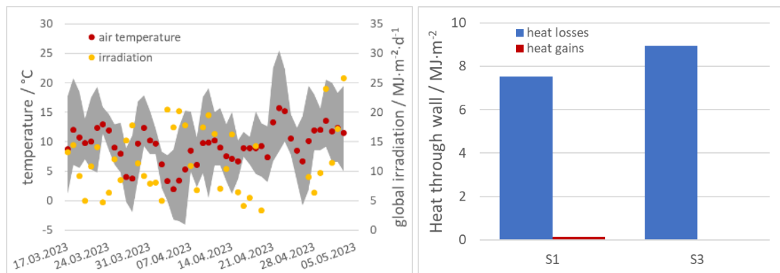
Fig. 9: Measured daily mean air temperature (red dots), minimum and maximum daily air temperature (grey area), and horizontal solar global irradiation (left); summarized heat gains and losses from March 17, 2023 to May 03, 2023 through the wall sections without LWS (right).
