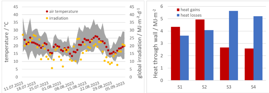
Fig. 4: Measured daily mean air temperature (red dots), minimum and maximum daily air temperature (grey area), and horizontal solar global irradiation (left); summarized heat gains and losses from July 11, 2023 to September 05, 2023 through the wall sections S1 and S2 without and S3 and S4 with LWS (right).
