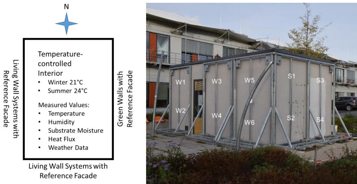
Fig. 2: Schematic plan view of the measurement setup for LWS on our outdoor test facility (left) and southwest view of the test facility with frames for the LWS and designations for the wall sections (right).
