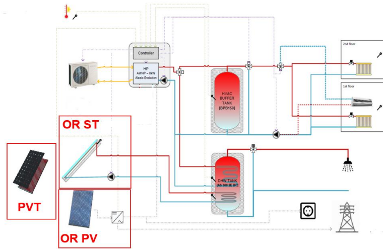
Figure 1: Building's energy systems configuration
