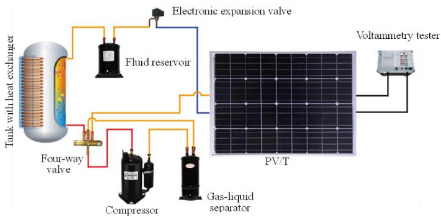
Fig. 3: PVT heat pump water heater
