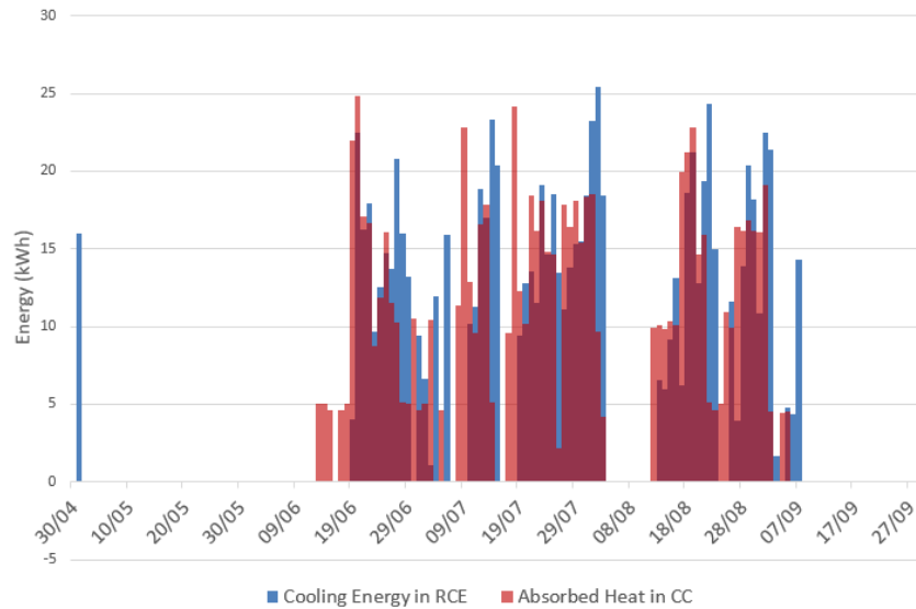
Fig 5. Visual comparison between the cooling energy produced in the RCE and the cooling energy consumed in the chilled ceiling.
