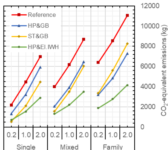
Figure 4: Comparison of the CO 2 -equivalent emissions of the four systems over the circulation load and the tapping profile calculated with expected CO 2 emission factors for electricity in 2030 (with UA factor of 1 and without return valve).
