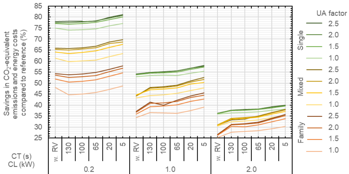
Figure 5: Illustration of the savings in CO 2 -equivalent emissions and energy costs of the solar thermal & gas boiler system compared to the reference system via the changeover time (CT) of the return valve and the circulation load (CL) (w. RV: without return valve).
