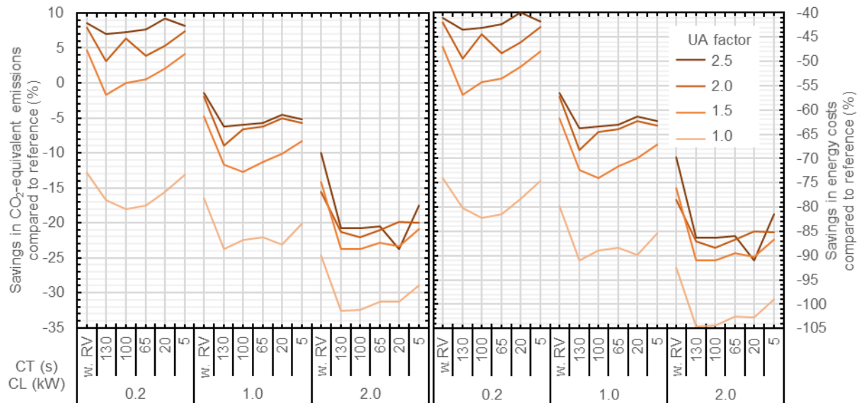
Figure 7: Illustration of the CO 2 -equivalent savings (left) and the energy cost savings of the heat pump & electric instantaneous water heater system compared to the reference system via the changeover time (CT) of the return valve and the circulation load (CL) with tapping profile Family.
