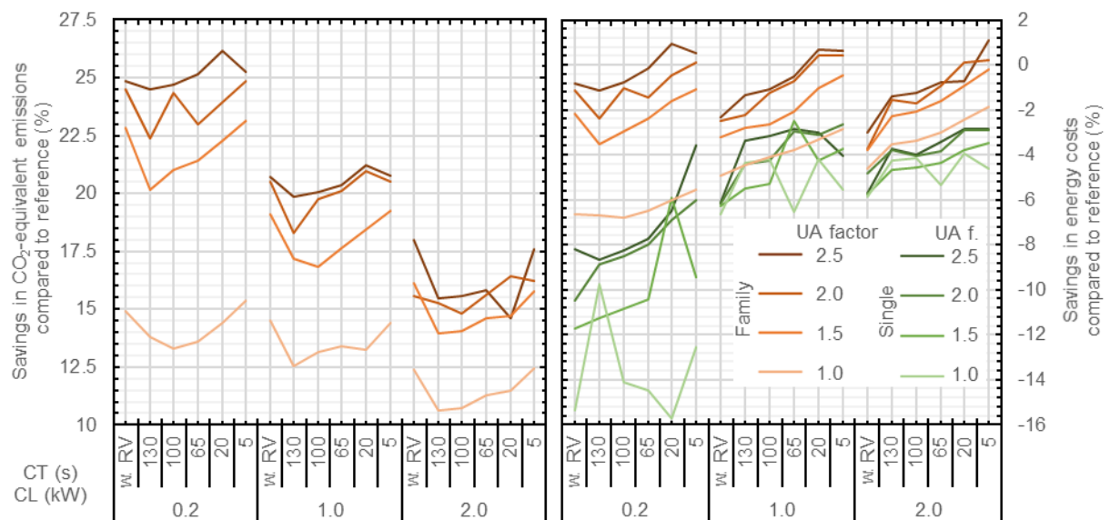
Figure 6: Illustration of the CO 2 -equivalent savings (left) and the energy cost savings of the heat pump & gas boiler system compared to the reference system via the changeover time (CT) of the return valve and the circulation load (CL) (w. RV: without return valve).
