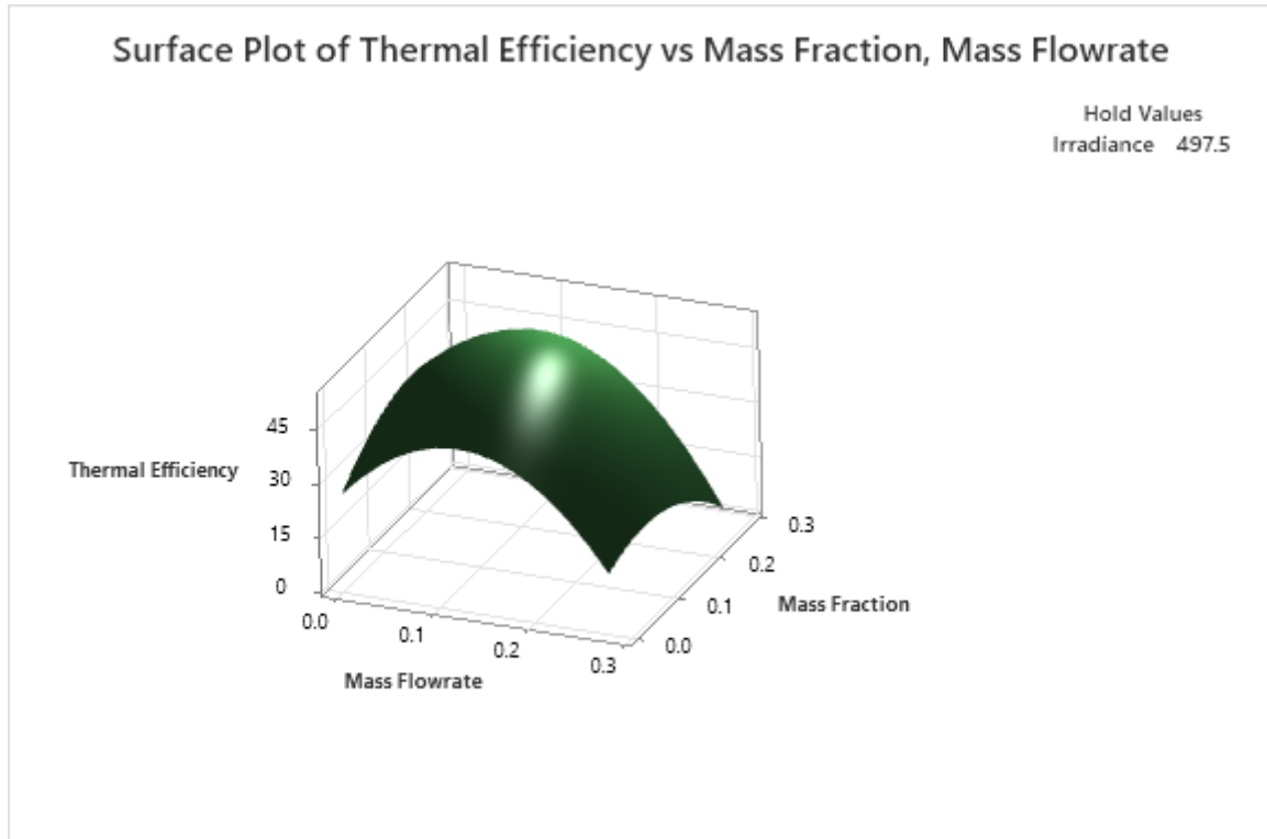
Figure 4: Surface plot of thermal efficiency generated with irradiance held constant at 497.5 W/ m 2 for CCD
