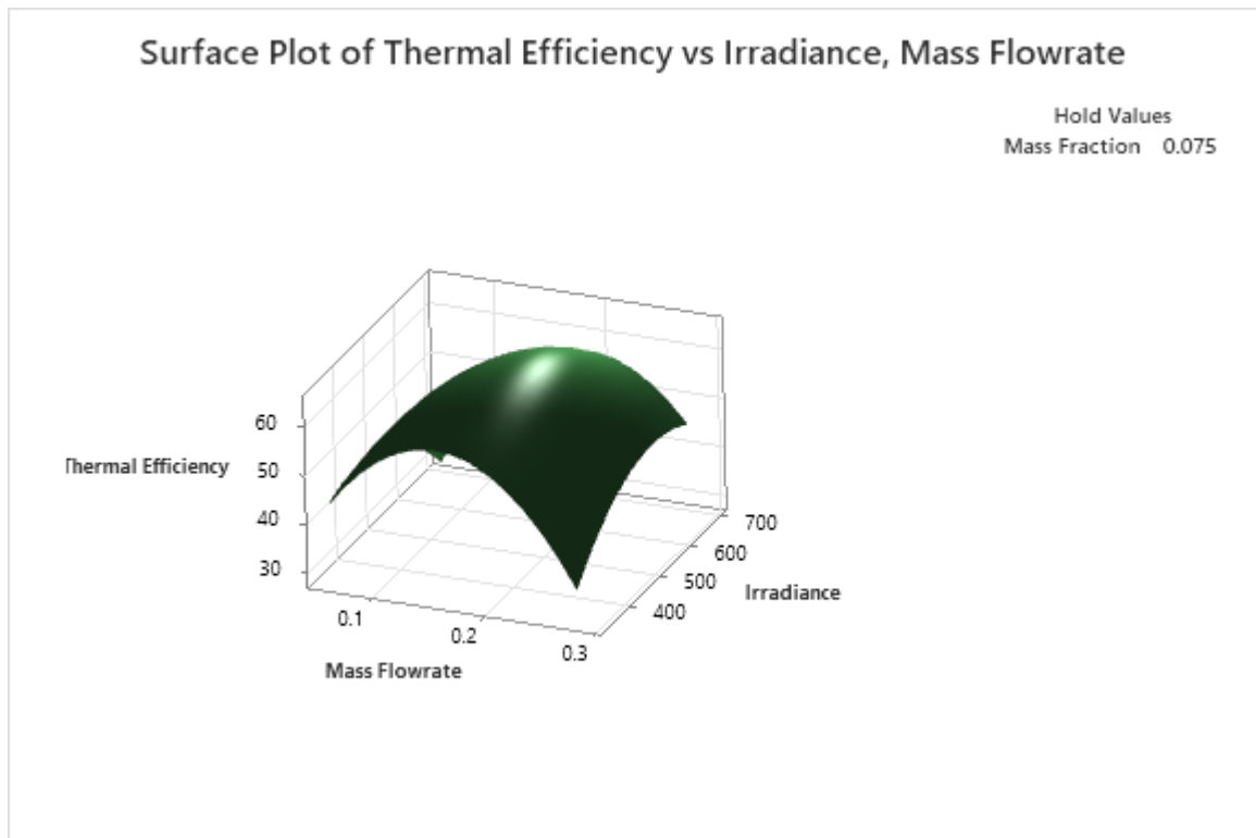
Figure 7: Surface plot of thermal efficiency generated with mass fraction held constant at 0.075% for BBD
