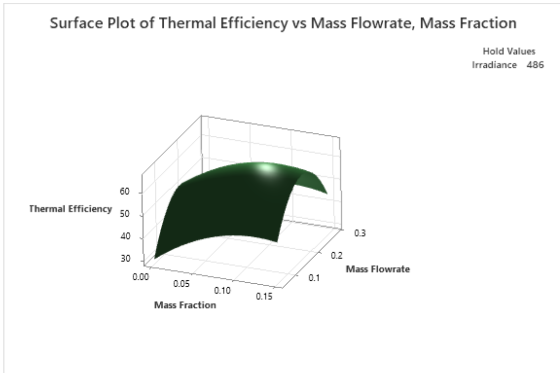
Figure 5: Surface plot of thermal efficiency generated with irradiance held constant at 486 W/ m 2 for BBD
