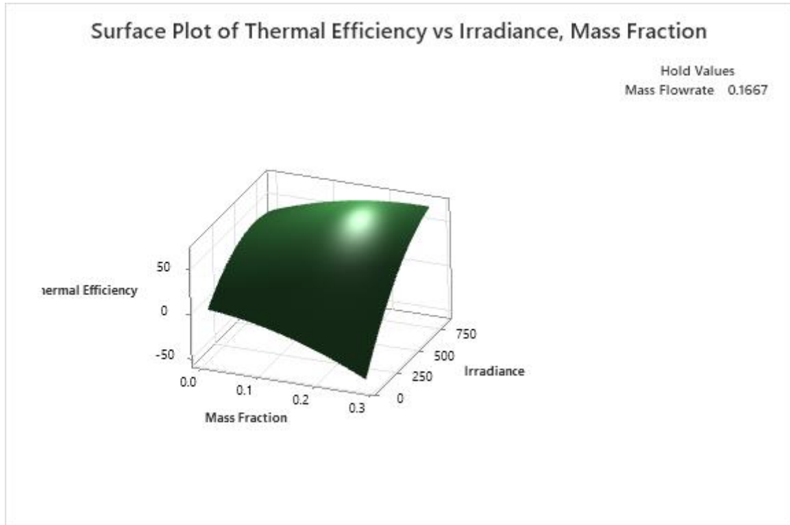
Figure 2: Surface plot of thermal efficiency generated with mass flowrate held constant at 0.1667 kg/s for CCD
