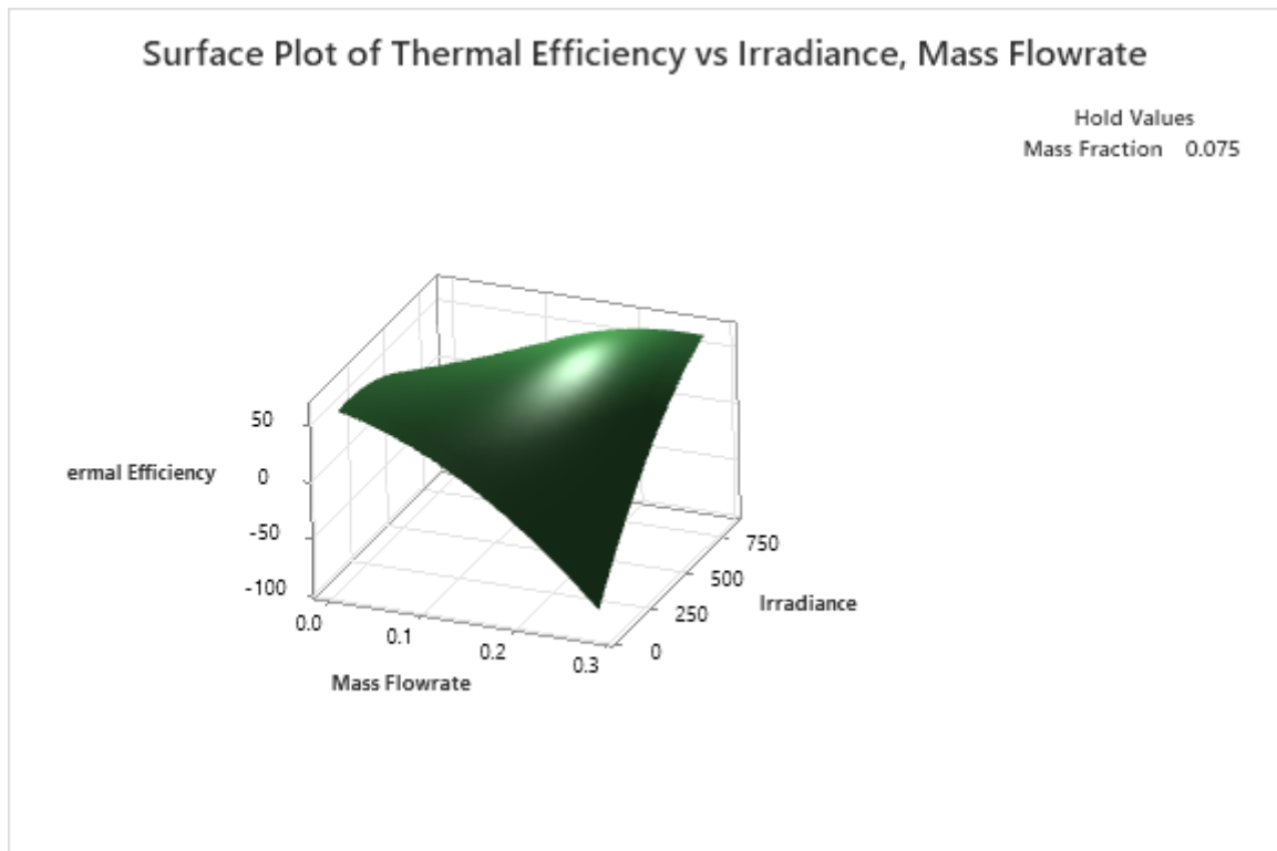
Figure 3: Surface plot of thermal efficiency generated with mass fraction held constant at 0.075% for CCD
