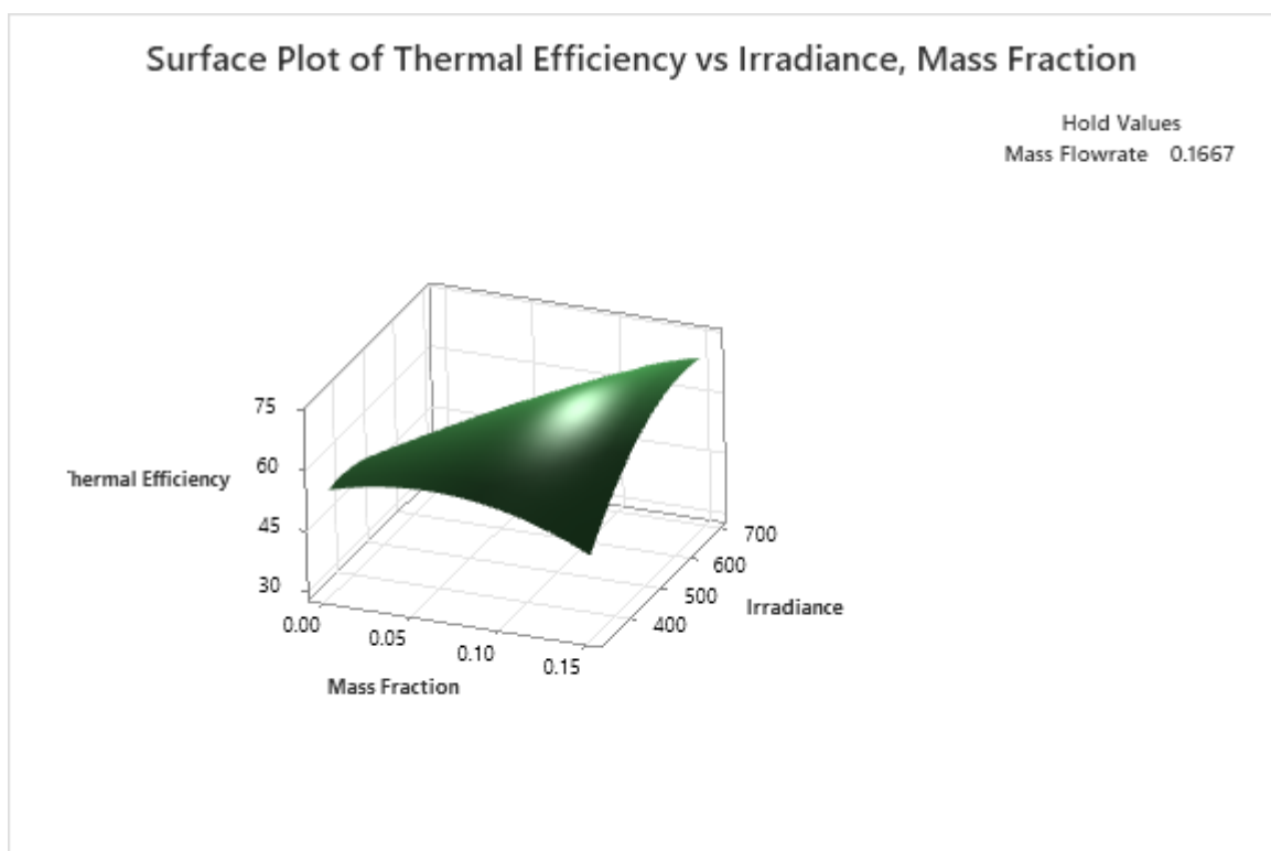
Figure 6: Surface plot of thermal efficiency generated with mass flowrate held constant at 0.1667 kg/s for BBD
