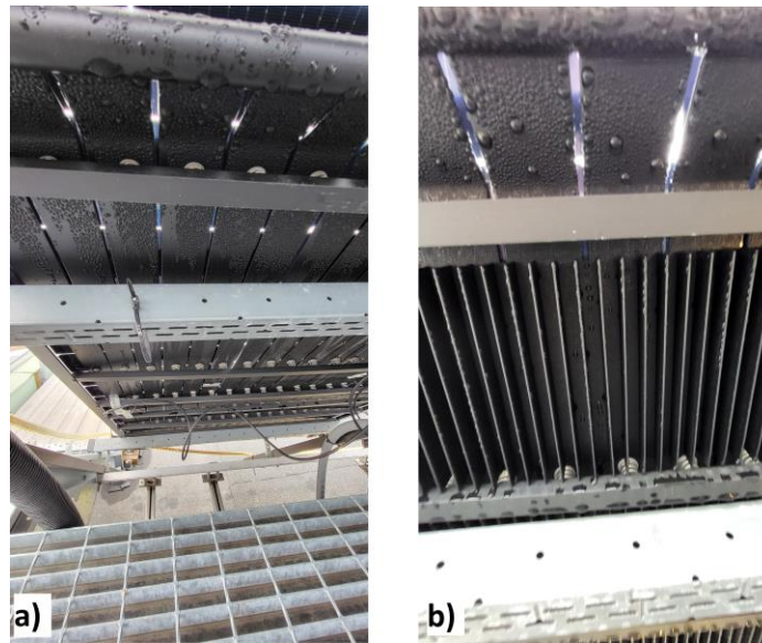
Fig. 3: Condensation forming on the collector surface for a) non-finned panel and b) finned panel.
