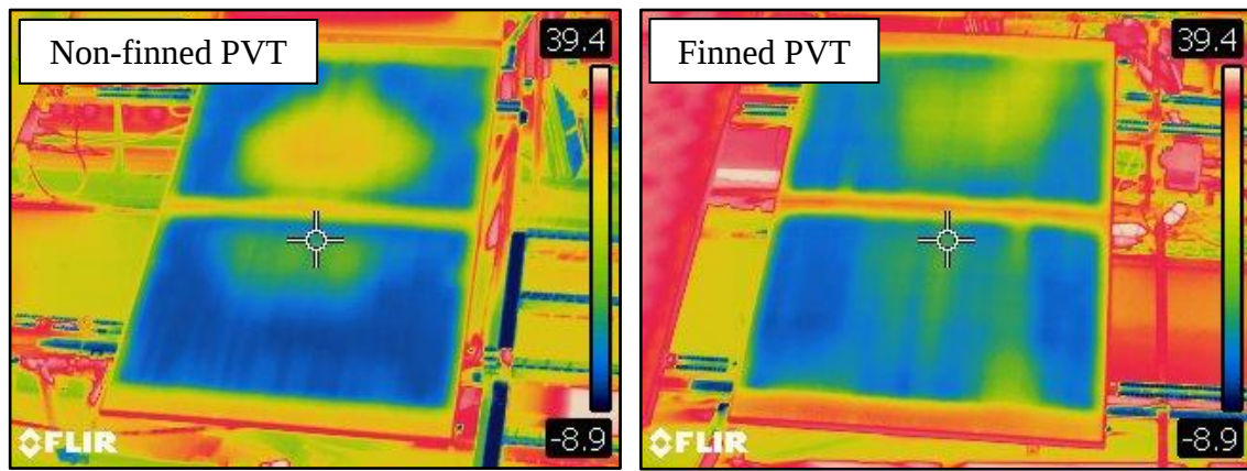
Fig. 8: Thermal images of the two PVT collectors (non-finned on the left and finned on the right) to show the imperfect thermal contact between the PV and the absorber, showing the larger airgap present in the non-finned PVT collector.
