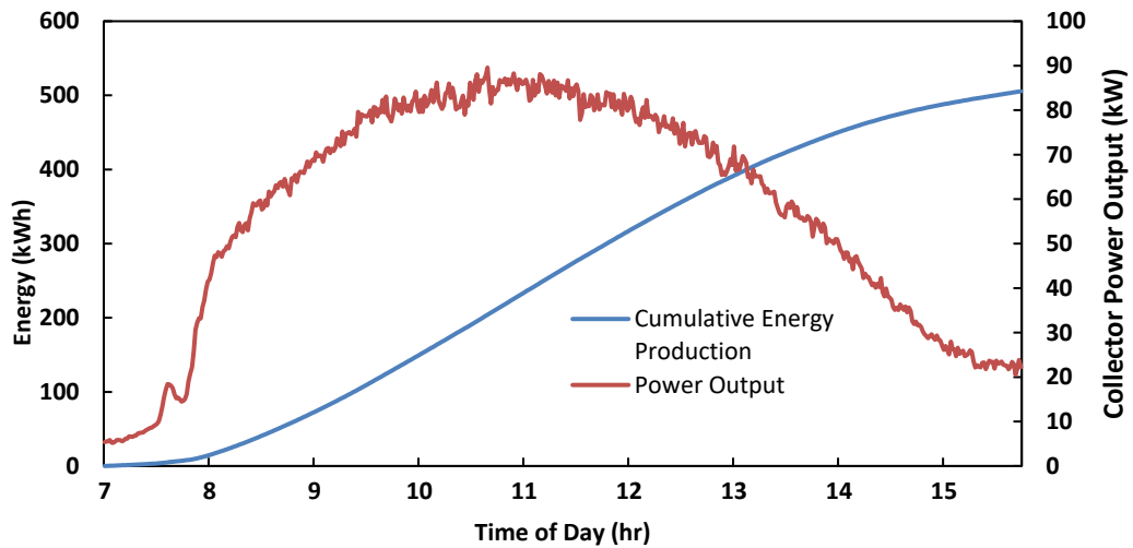
Fig. 12: Cumulative energy and power measured over the course of March 23rd, 2024
