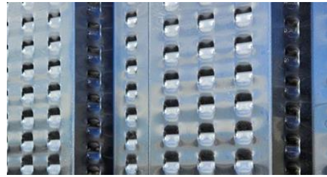
Fig. 1: Closeup of perforated aluminum selective surface.
