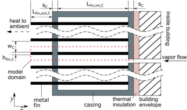
Figure 12: Design scheme of the condenser (cross-section top view). The scheme is not to scale as the width in y-direction is approximately 1.1 m, while the depth in z-direction is only approximately 9 cm. (Boeckmann et al. 2024)
