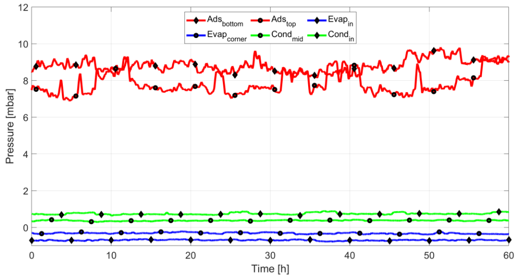
Figure 8: Evolution of the absolute pressures inside the three components adsorber (red), condenser (green) and evaporator (blue) over time during the initial leak tests.
