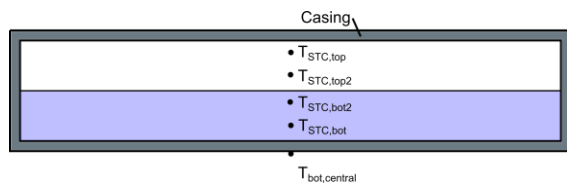
Figure 13: Cross-section side view of the evaporator with installed temperature sensors. Four sheath thermocouples are fed into the evaporator and one thermocouple is installed centrally at the outside of the bottom.
