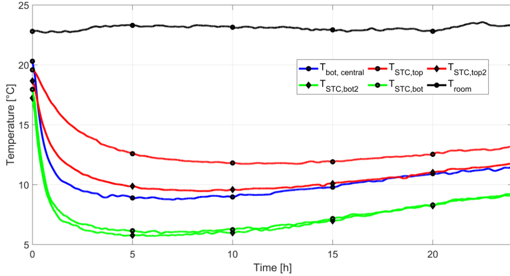
Figure 9: Evolution of temperatures at the central outer bottom (blue), inside the evaporator and inside the room (test chamber, black) over time during the 24h commissioning test.
