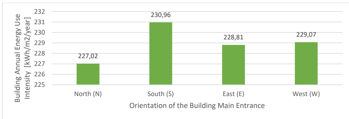
Fig. 2: Building annual energy use intensity according to the orientation of the building main entrance
