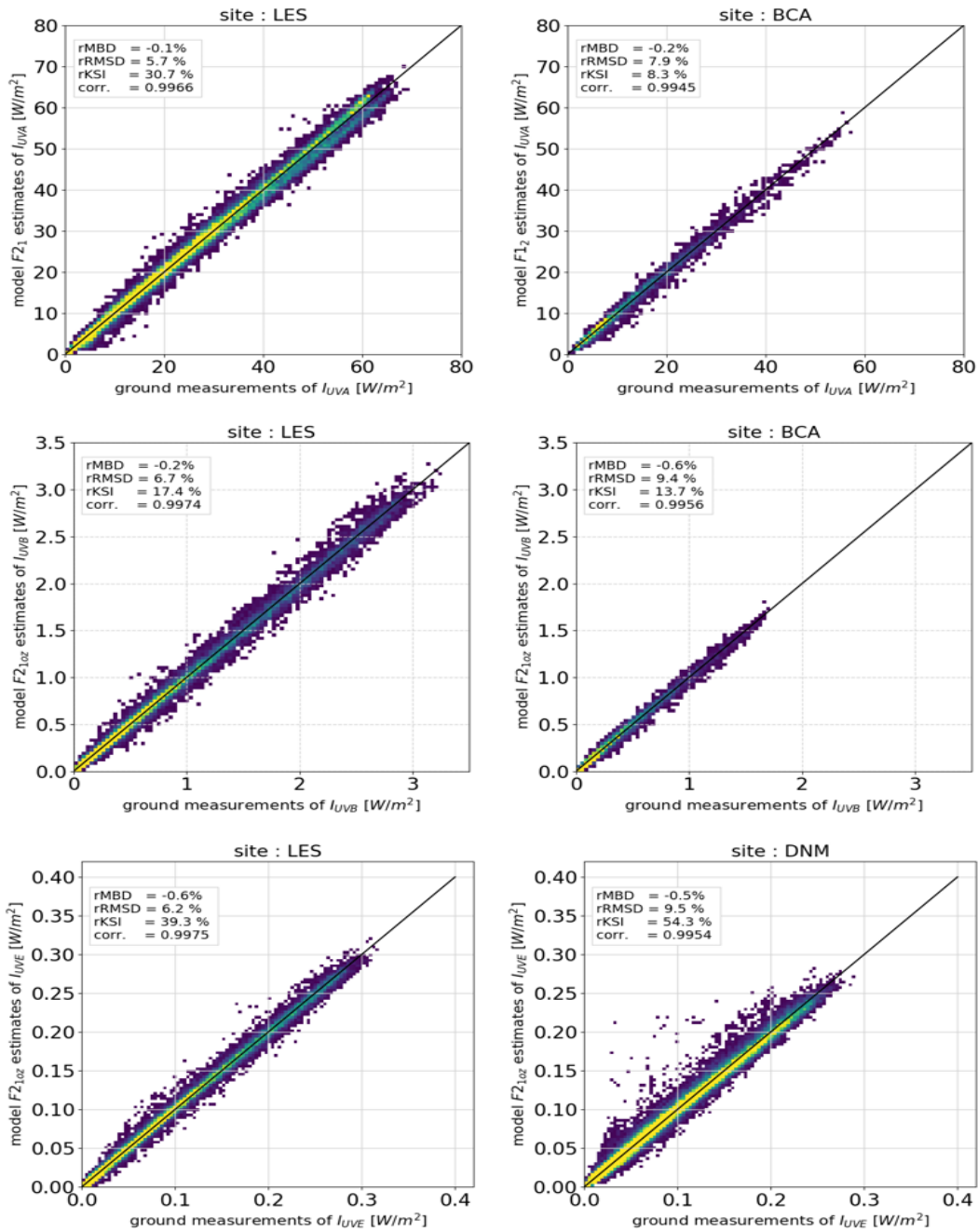
Fig. 3: Scatter plots of the best models for each band. In the first row correspond to UV-A, the middle and bottom row corresponds to UV-B and UV-E respectively.
