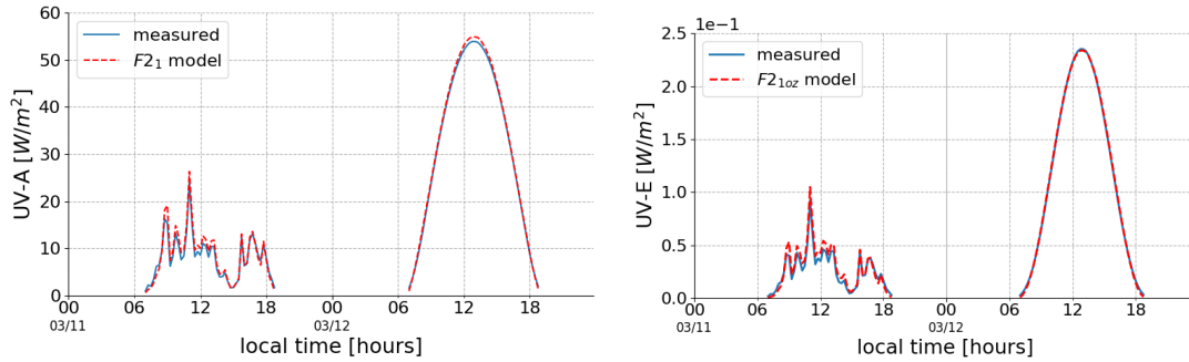
Fig. 2: F2 models estimates for the UV-A and UV-E bands vs time for a cloudy day and a clear day at the LE site.
