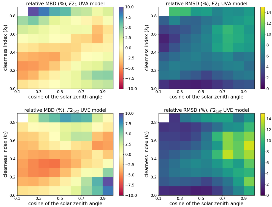
Fig. 4. rMBD (left) and rRMSD (right) distributions vs the cosine of the solar zenith angle and the clearness index at the LES site. Upper panels are for the to UV-A band and the lower panels for UV-E estimates.
