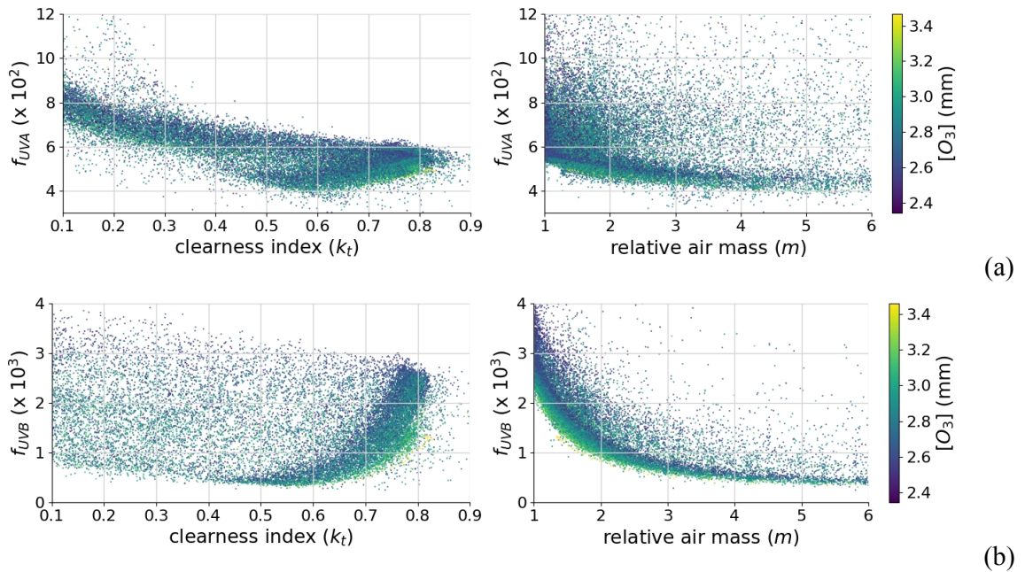
Fig.1: UV fraction vs clearness index and air mass (data from LES site). (a) UV-A fraction and (b) UV-B fraction are shown. Data is colored according to Ozone concentration, [O_3] . The dependence of f_{UVB} with Ozone concentration appears clearly. The behavior of f_{UVE} is similar to f_{UVB} (not shown).
