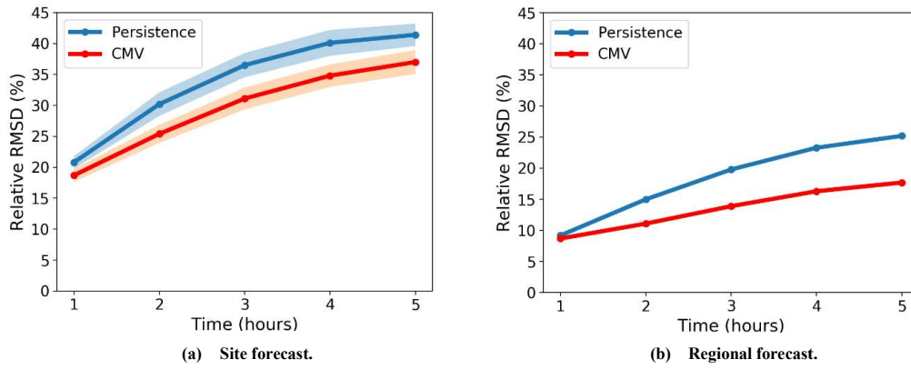
Fig. 2: Relative RMSD performance metric vs time horizons.
