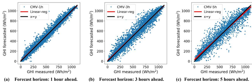
Fig. 4: Scatter plots between the CMV predictions and the measurements for different time horizons (regional forecast).
