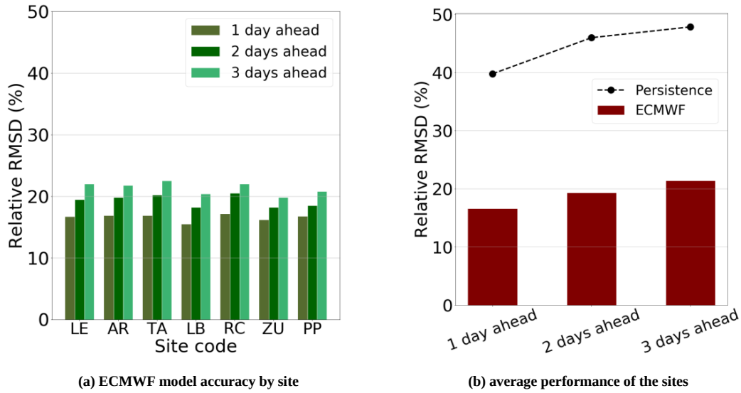
Fig.3: Performance model daily forecast.
