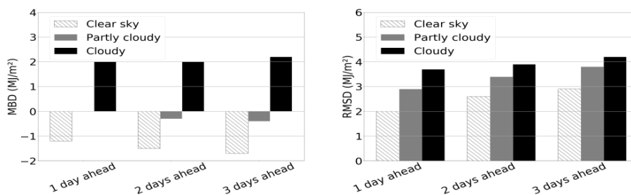
Fig.4: Daily-integrated performance evaluation discriminated by sky condition.
