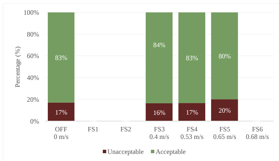
Figure 10: Results of fan-speed setting preference survey during the testing of the control sequence
