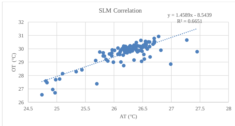
Figure 5: Straight Line Method correlation between OT and AT
