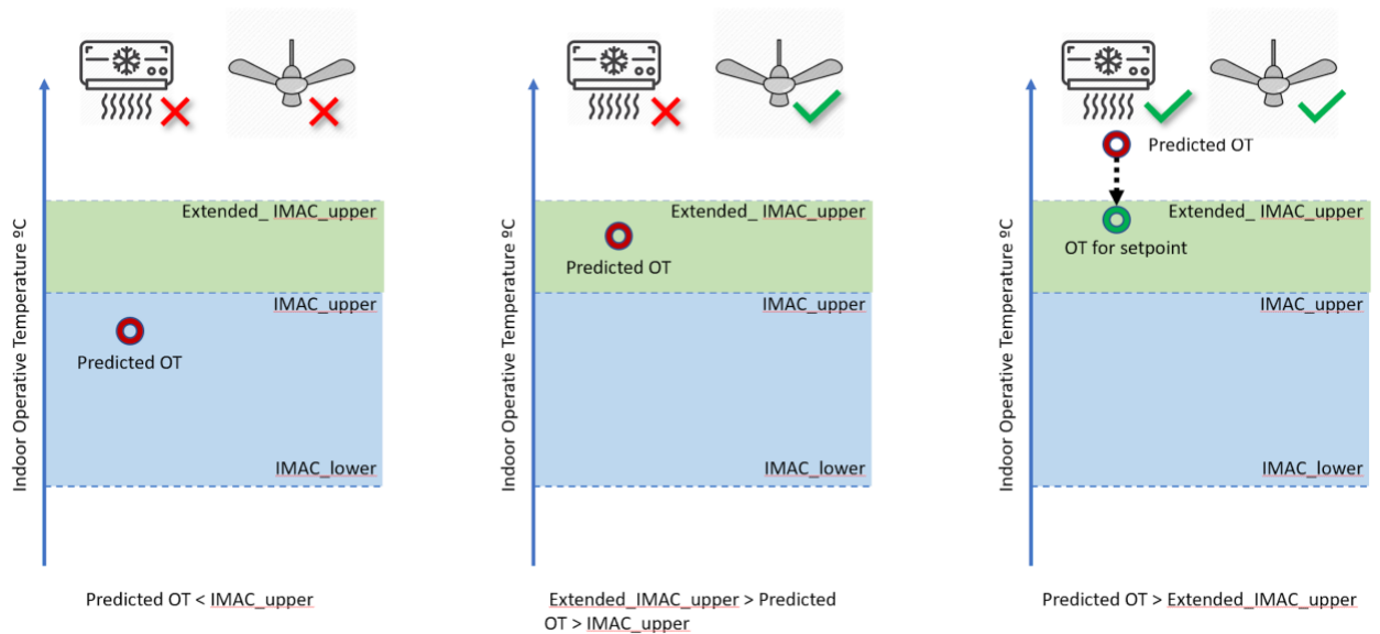
Figure 3: Three scenarios for the control sequence
