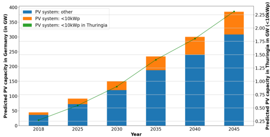
Fig. 6: Predicted capacity of rooftop PV system ( <10 \text{ kW}_p ) in Thuringia (left y-axis: green line) until 2045
