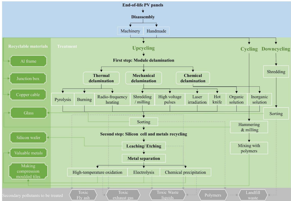
Fig. 5. Possible EOL PV panels recycling strategies and process [7].
