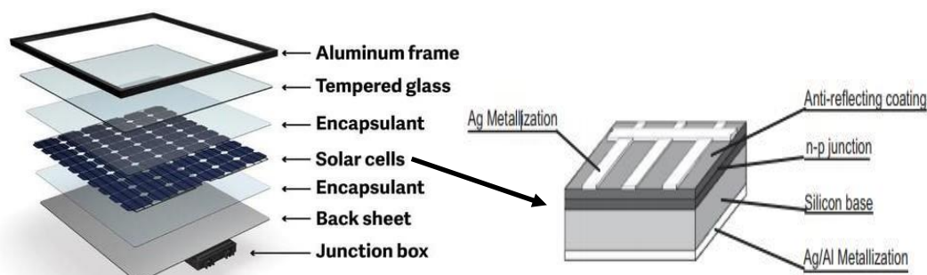
Fig. 1. Solar module basic structure and types of material used in solar cells [Dias, P, et. al. 2017].
