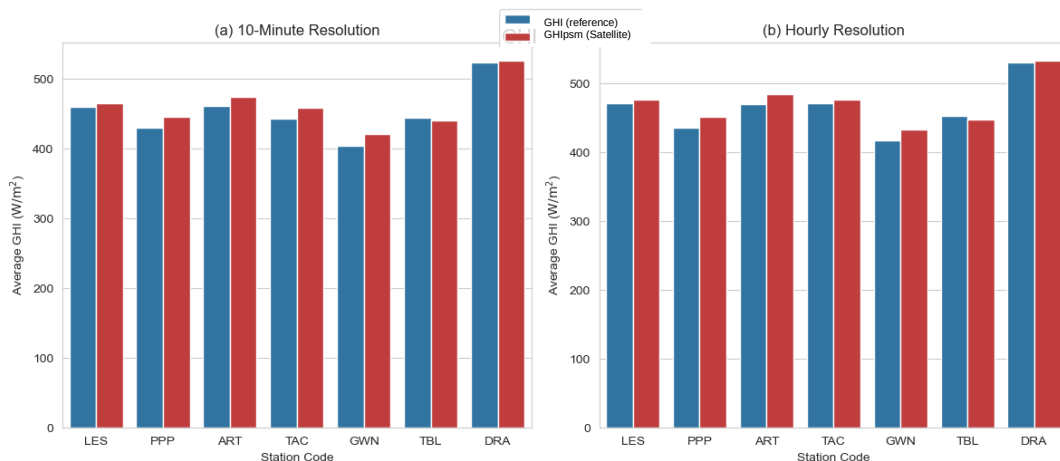
Figure 2. Mean Global Horizontal Irradiance (GHI) across Sites. GHI values derived from the ground measurements (blue) and PSM model (GH Ipsm ) estimates (red). (a) 10-Minute Resolution and (b) Hourly Resolution.
