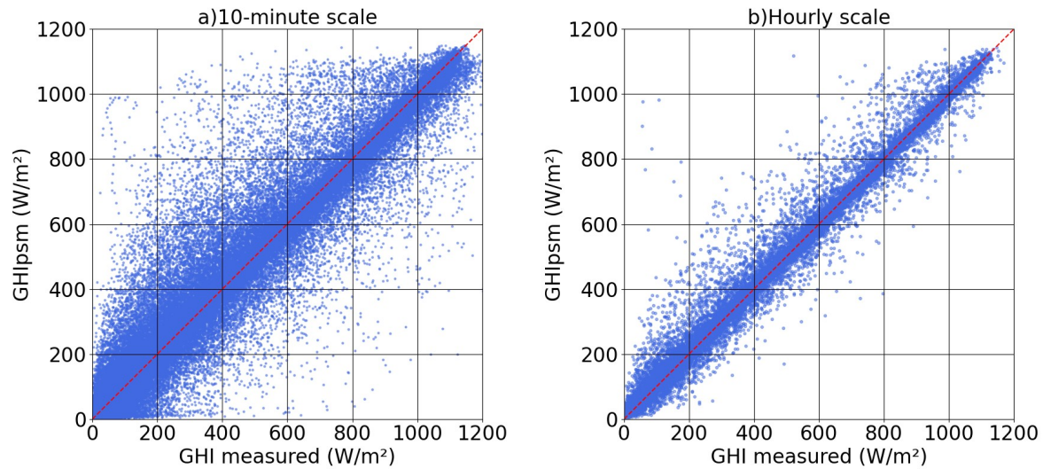
Figure 4. Scatter plots of the PSM model estimated GHlpsm versus GHI measured at the Artigas (ART) station. (a) Data with 10-minute time resolution, (b) hourly mean data. The red dashed line indicates the 1:1 reference line.
