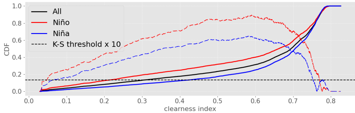
Figure 3. CDF of daily clearness index (kt) during November–December by ENSO phase. Dashed lines show the absolute difference with the ALL curve (scaled \times 10 ). The threshold 0.0134 indicates significant difference at 1% level.
