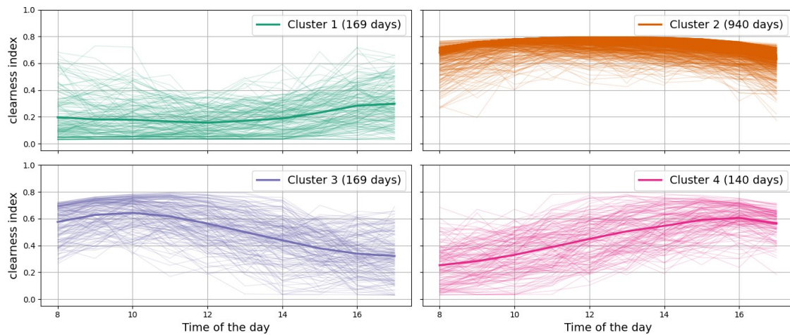
Figure 5. Daily kt profiles grouped into four clusters: Cluster 1 (OC), Cluster 2 (CL), Cluster 3 (CL-AM), Cluster 4 (CL-PM). Thin lines represent individual days, while the thicker line shows the mean profile of each cluster.
