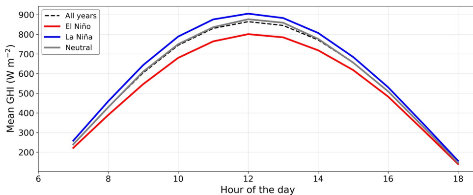
Figure 2. Mean hourly GHI profiles during November–December for El Niño (red), La Niña (blue), and neutral (grey) years. The dashed black line indicates the climatological mean (all years).
