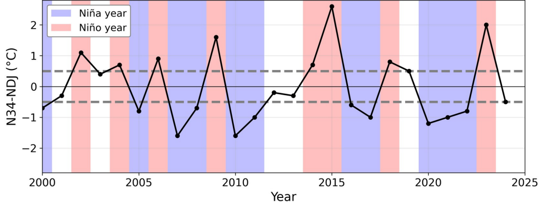
Figure 1. Evolution of the N3.4 index for the November-December-January (NDJ) season during 2000-2025. Shaded colors indicate the ENSO phase for each year: El Niño (red), La Niña (blue), and neutral (white).
