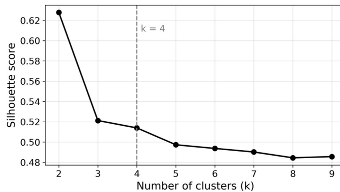
Figure 4. Silhouette score as a function of the number of clusters ( k ). The vertical dashed line indicates the selected value ( k = 4 ), chosen as a trade-off between clustering performance and physical interpretability.
